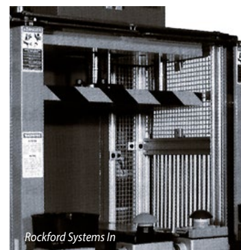
Photoelectric "light curtain" on a hydraulic press.
